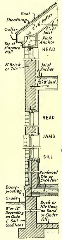
Wall Section
